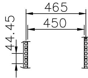
Mounting Dimension
